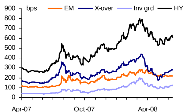
Fig 2: CDX spreads
